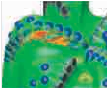
Using CFD to visualize flow patterns enables designers to analyze how design modifications affect bit performance and choose the optimal solution.
