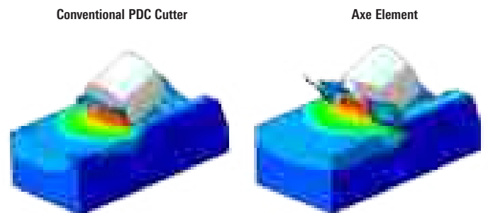
FEA testing showed that the Axe element achieves at least 22% deeper penetration compared with conventional PDC cutters under the same drilling conditions and parameters.
