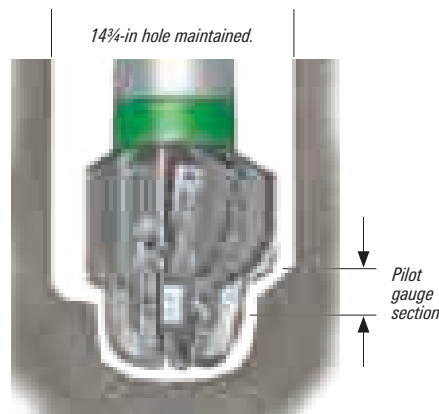
12 1/4 in x 14 3/4 in QDS7213.
